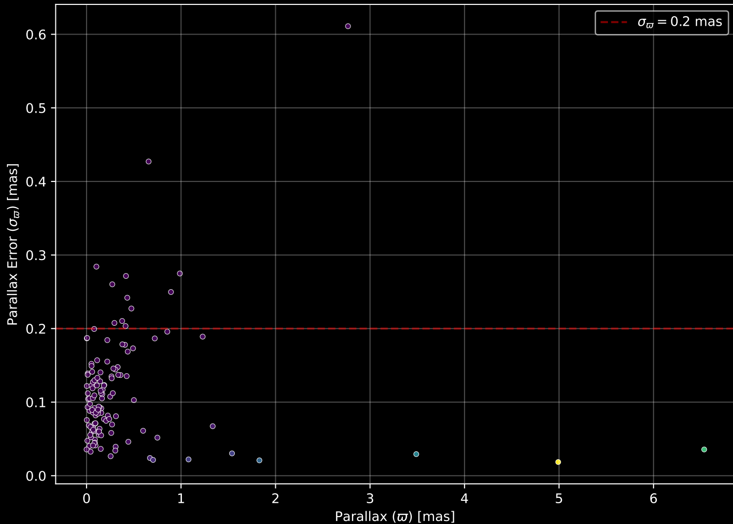
APOGEE DR17 Field: [357+03-O] Parallax Quality (n= 129)
