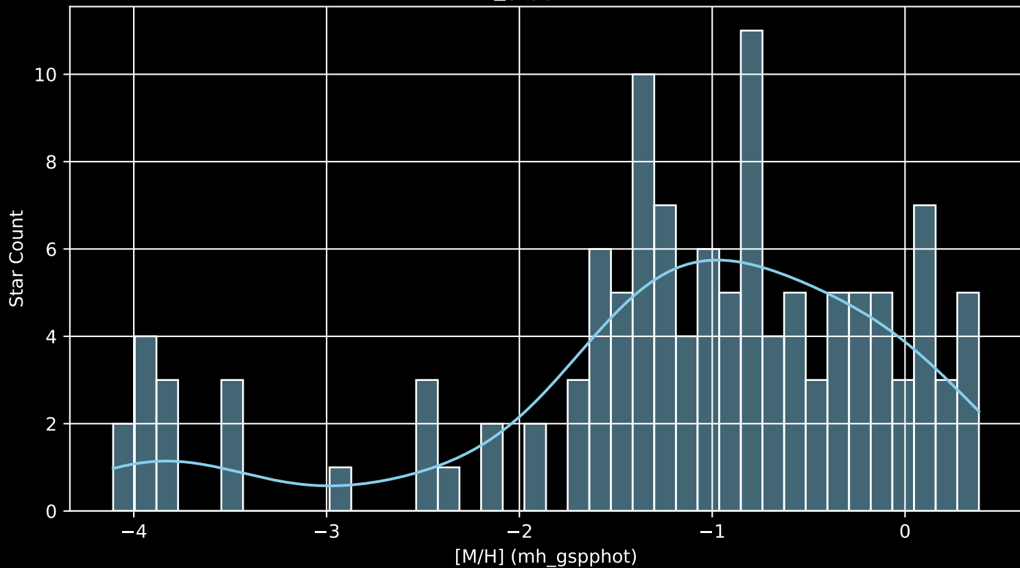
APOGEE DR17 Field: [357+03-O [M/H] (mh_gspphot) (n= 123)
