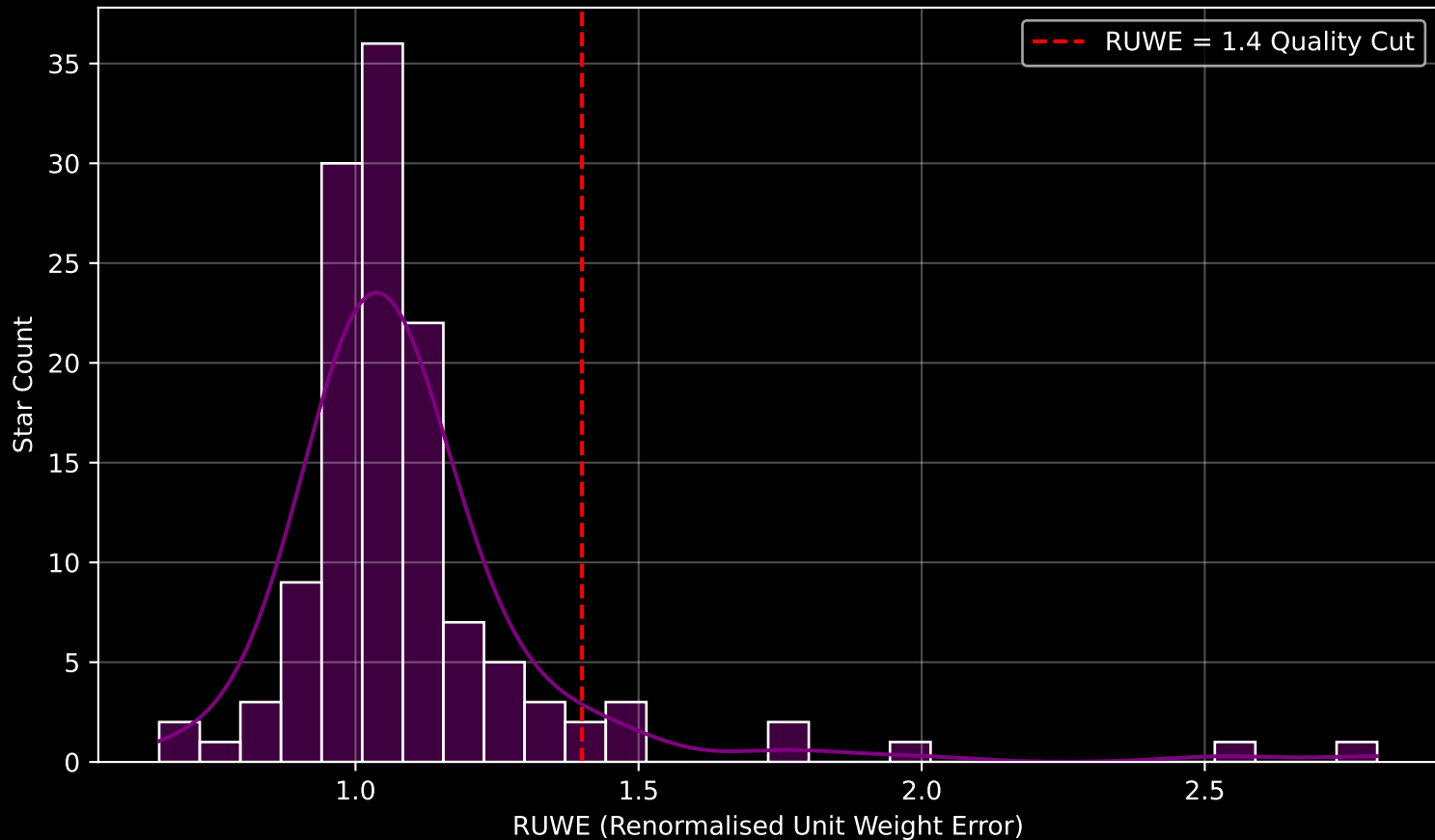
GAPOGEE DR17 Field [357+03-O] RUWE Distribution (n= 128)
