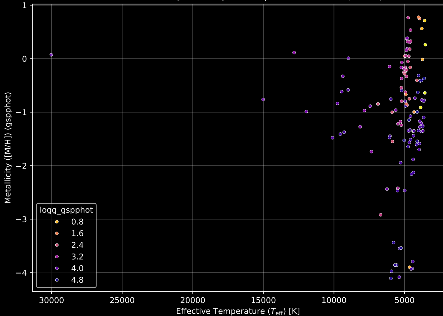
APOGEE DR17 Field: [357+03-O] Stellar Population Parameters (n= 129)
