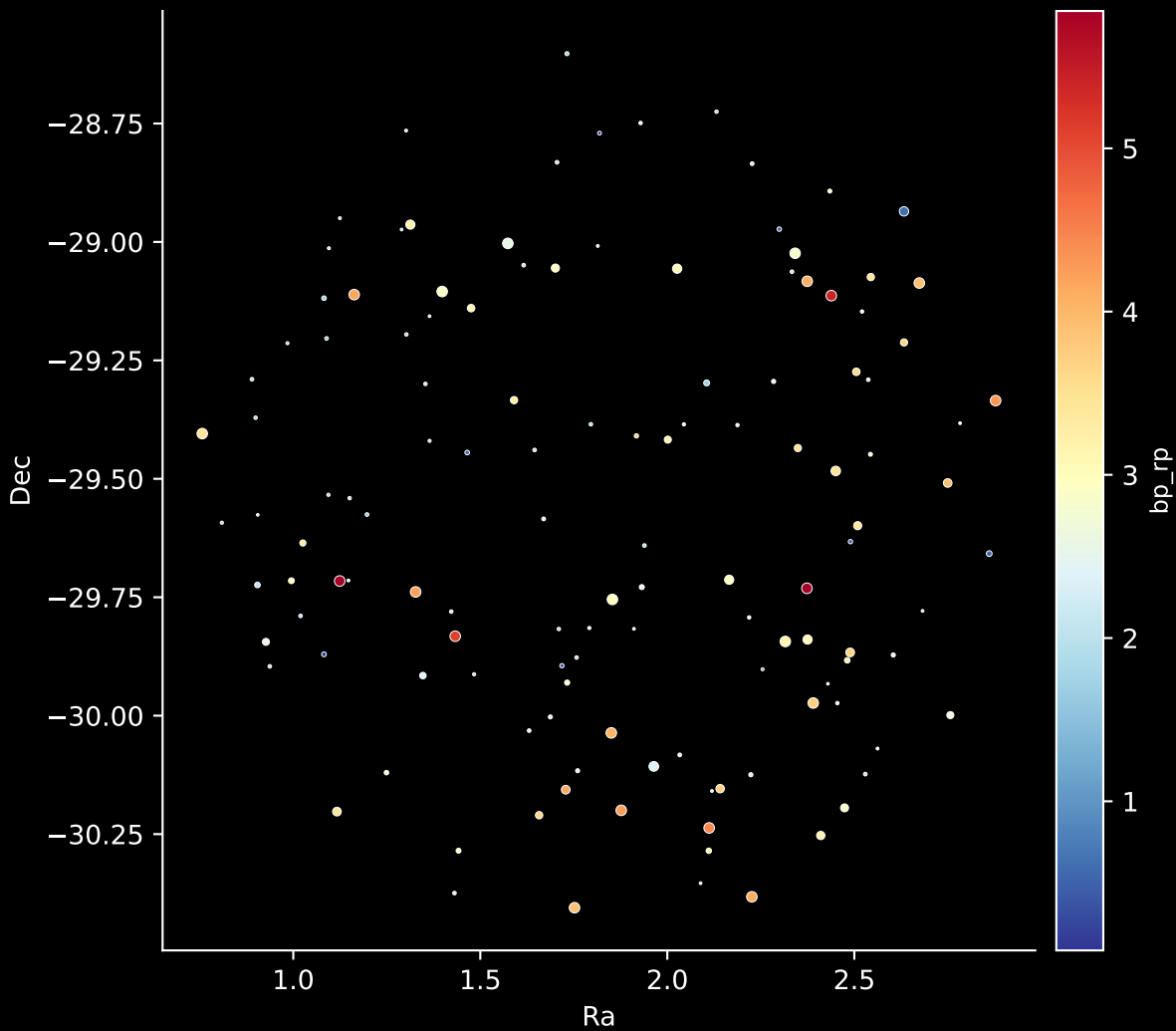
APOGEE DR17 Field: [357+03-O] Stars: 129
