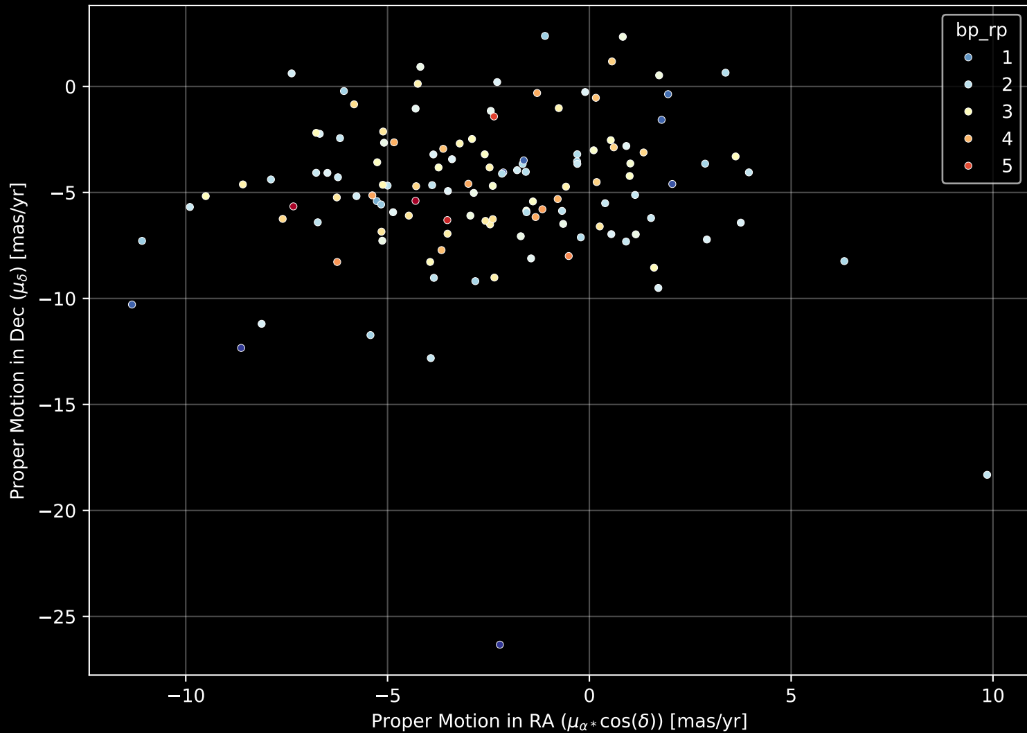
APOGEE DR17 Field: [357+03-O] Proper Motion Diagram (n= 129)
